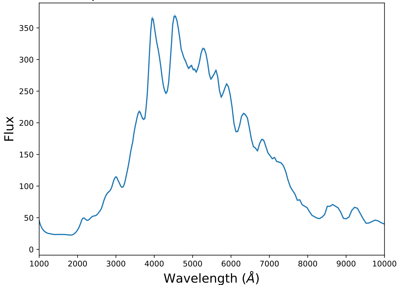
Spectrum 4 for transient SNIax at z=0.49
